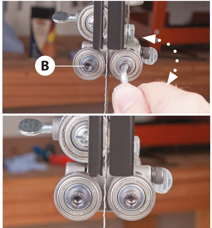
Guide bearings set to 0.5 thickness to the blade
